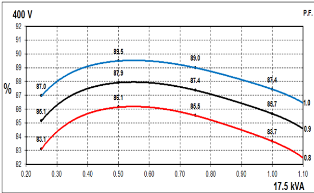
50Hz Curves
