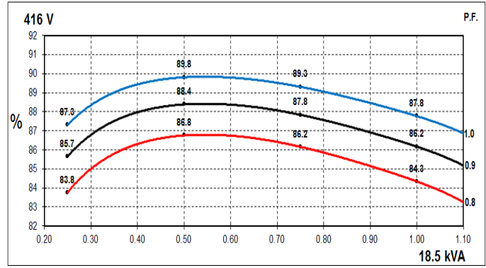
60Hz Curves
