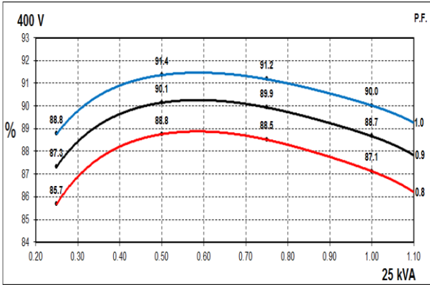
50Hz Curves
