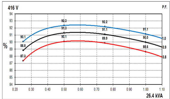
60Hz Curves
